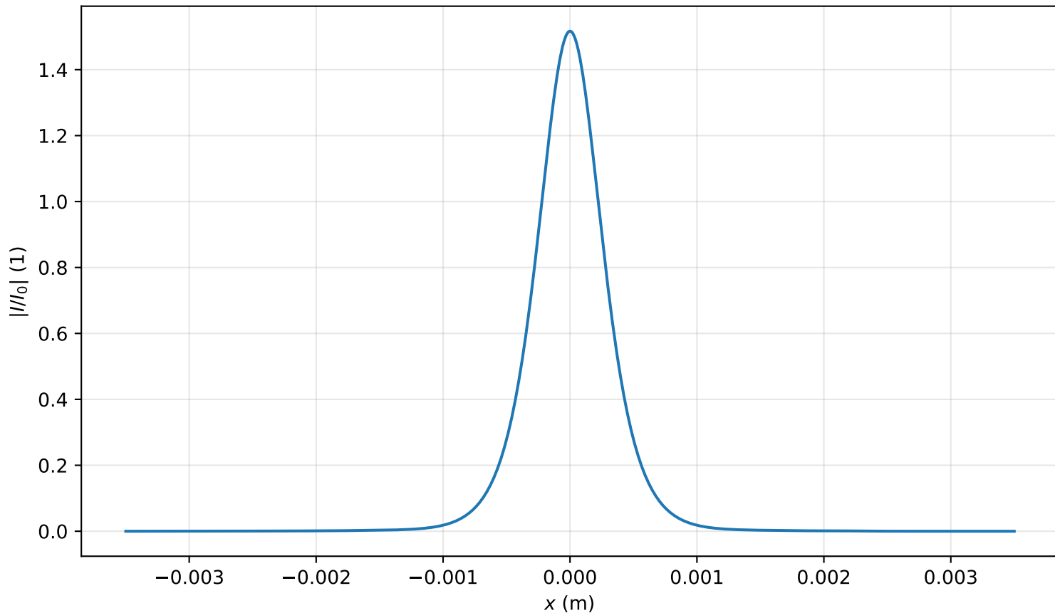
Intensity profile I(x, y = 0, z = 3.344m)/I_0 , P_{in}=0.9P_{cr} , artificial time
